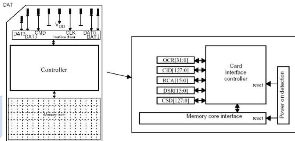
Figure 3-1 SD Card Pin assignment
