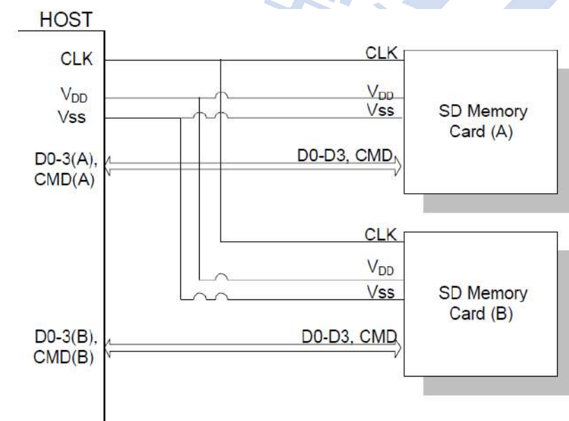
Figure 3-2 SD Memory Card System Bus Topology
