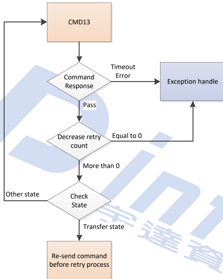
Figure 7-3 Retry Error Handling Process
